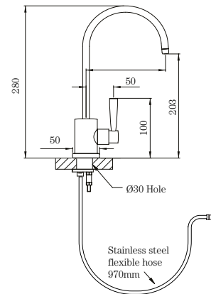
AU.1601 - Contemporary filter tap to suit Orbicq, Oberon, Mimas, and Io taps
