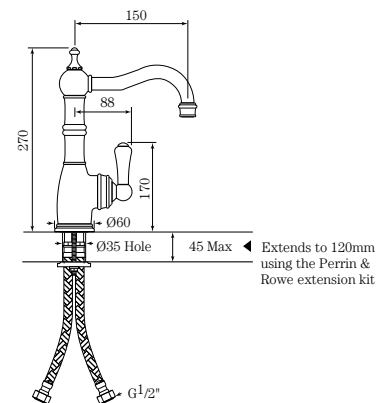
AU.4739 - Aquitaine bar sink tap with metal lever (short reach spout)
